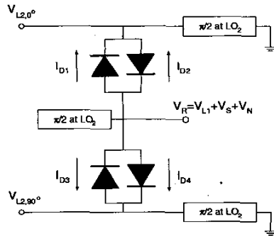
Figure 4 - Mixer diode currents
