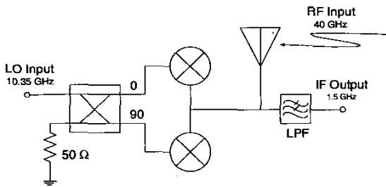
Figure 3 - 4th harmonic mixer using antiparallel diode pairs
