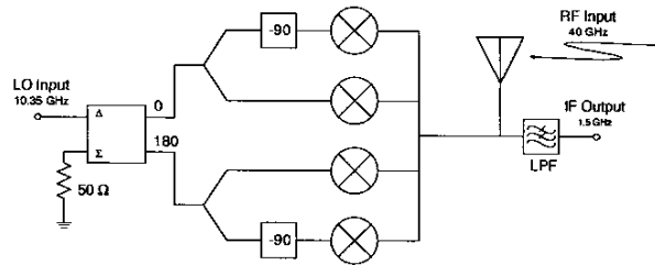
Figure 5 - Biasable 4th harmonic diode mixer
